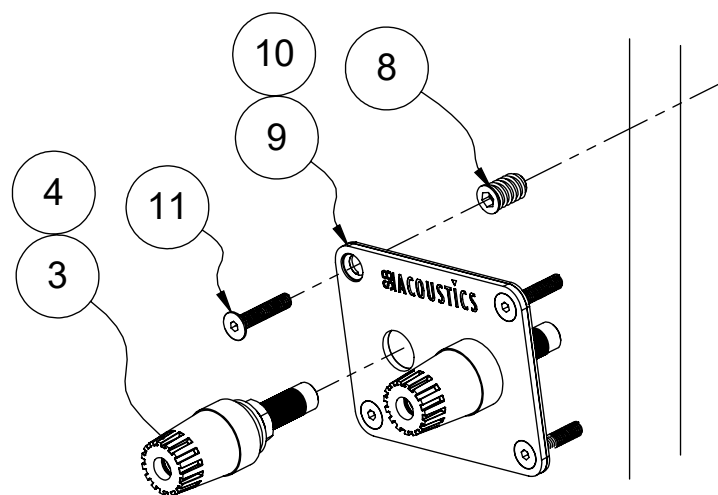
DETAIL C SCALE 1 : 2
